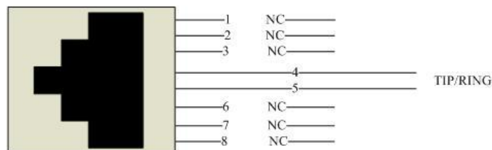
Figure 3: A400P Phone Jack Wire
