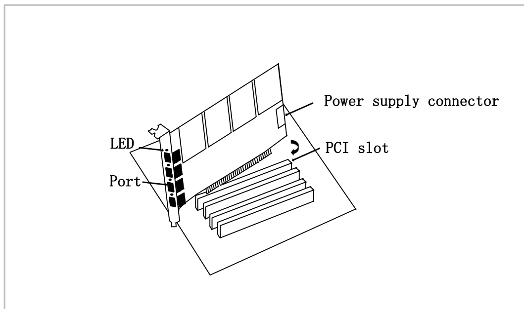
Figure 4 Hardware setup
