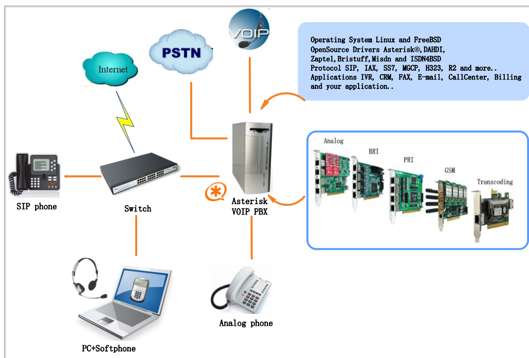
Figure 1 Topology
