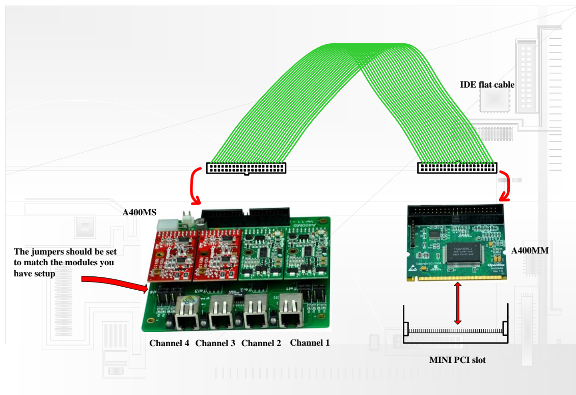
Figure 2 Hardware setup
